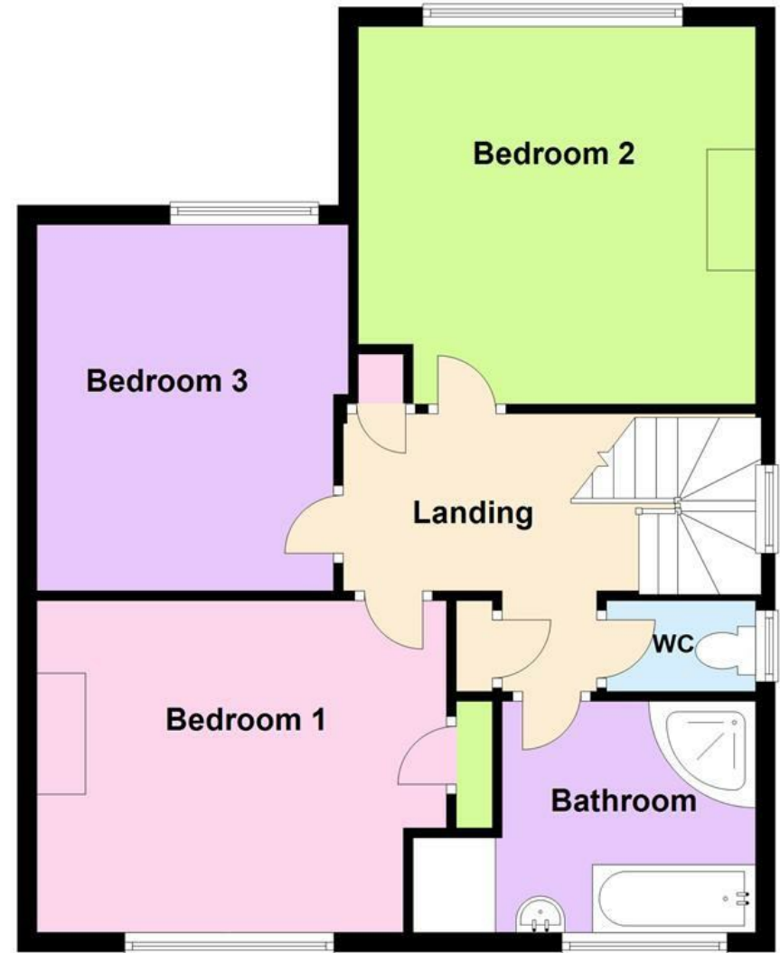
First Floor
